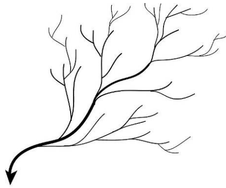
Dendritic Drainage Pattern
